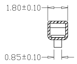
SEC:C-C
